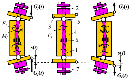
Fig. 10 Scheme of cyclic bending of the stud-nut connection: 1 – stud, 2 – nut, 3 – twisted support, 4 – intermediate detail, 5 – roll, 6 – four strain gauges, 7 – auxiliary nut; G_f(t) – force varying during loading cycle time t
