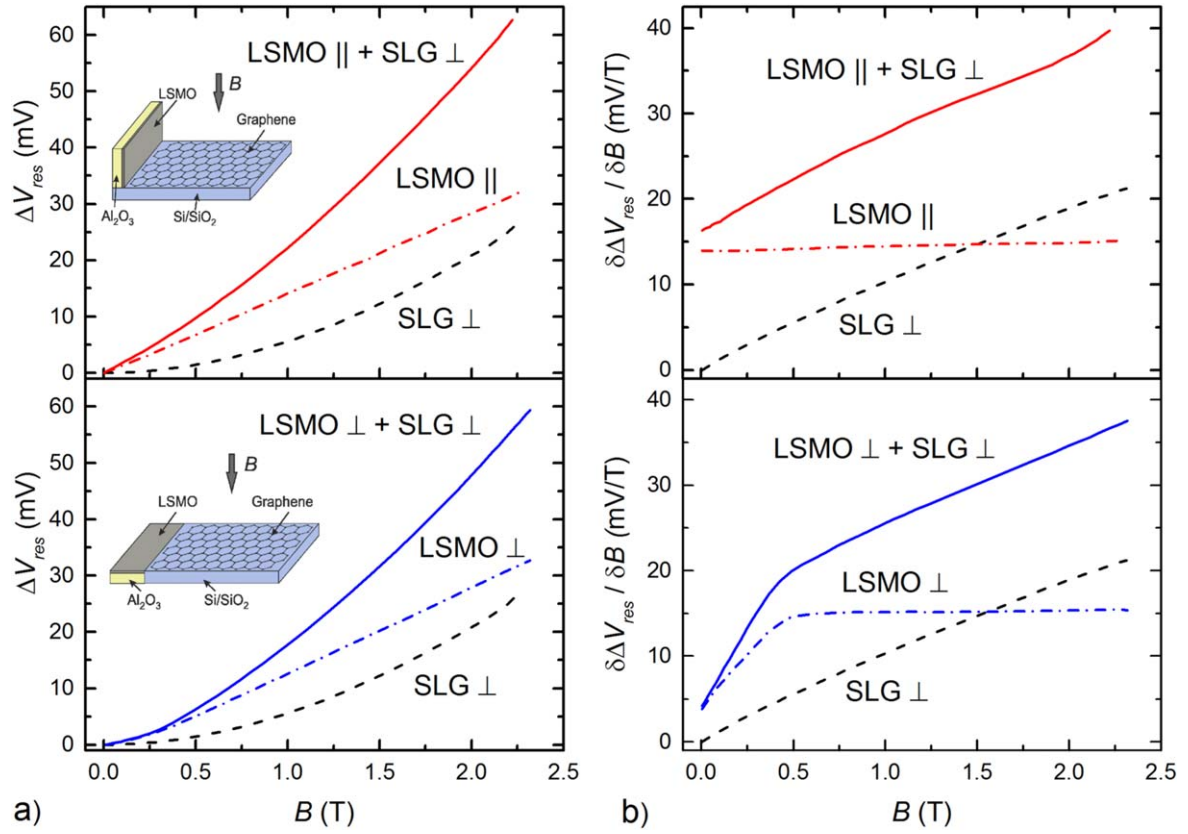
Figure 3. (a) The voltage response change \Delta V_{res} dependence on magnetic flux density B for hybrid GM sensor, when magnetic field is applied perpendicular to graphene layer and parallel to manganite film (upper graph, solid red line) or perpendicular to both graphene and manganite planes (lower graph, solid blue line). The dashed black curve represents voltage response change from individual graphene sensor ( SLG \perp ), while dashed–dotted lines represent voltage response from individual manganite sensor when magnetic field was applied parallel ( LSMO \parallel ) or perpendicular ( LSMO \perp ) to the film plane. (b) The sensitivity S of different sensors obtained from corresponding curves presented in graph (a). Power supply voltage V_s = 1.249 V, ambient temperature T = 294 K.
