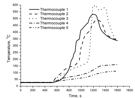
Fig. 14. Fragment 3.4 temperature changes
