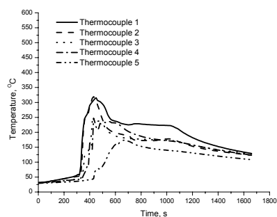
Fig. 10. Fragment 2.1 temperature changes
