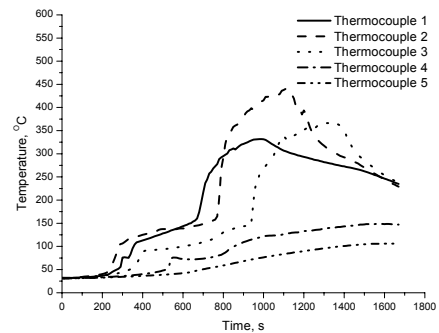
Fig. 11. Fragment 3.1 temperature changes
