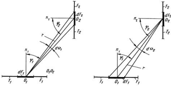
Fig. 1. The scheme of heat exchange by means of thermal radiation between two fields haphazardly located in space
