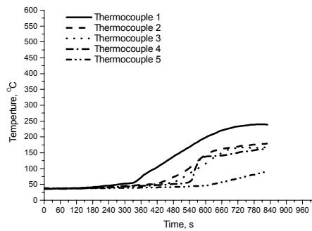
Fig. 7. Fragment 1.1 temperature changes
