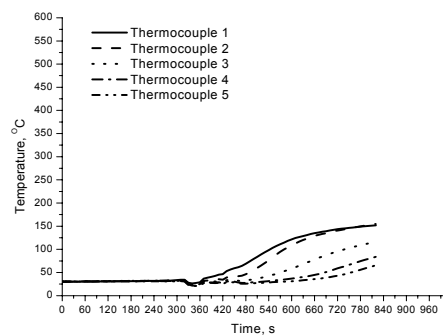
Fig. 8. Fragment 1.2 temperature changes
