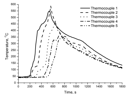
Fig. 12. Fragment 3.2 temperature changes
