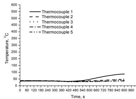
Fig. 9. Fragment 1.3 temperature changes
