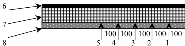
Fig. 3. Principal scheme of fragment tested: 1–5 – thermocouples, set in the non-combustible foundation, 6 – roof covering, 7 – thermal insulation, 8 – non-combustible
