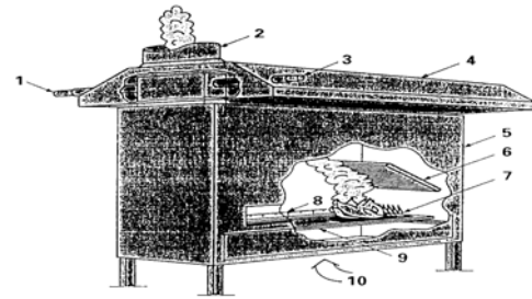
Fig. 4. Basic scheme of the equipment: 1, 3 – aperture (if projected); 2 – vent pipe; 4 – vent hood; 5 – test chamber; 6 – the screen surface of heat flux radiation; 7 – flame controlling burner; 8 – scale; 9 – specimen holder with the specimen; 10 – environment air suction through the bottom of the chamber
