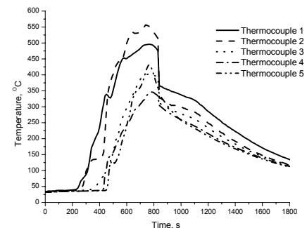
Fig. 13. Fragment 3.3 temperature changes
