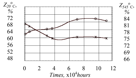
Fig. 8. Dependence of area reduction on time of operation: o – the research was done at the 20 °C temperature, × – the researches was done at the 545 °C temperature
