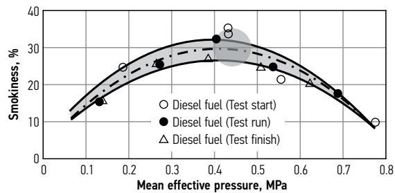
Fig. 3. The dependence of the smokiness SM of 1Z diesel engine on mean effective pressure P_{me} when the engine runs on diesel fuel
