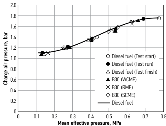
Fig. 6. The dependence of the charge air pressure P_K of 1Z diesel engine on mean effective pressure P_{me}
