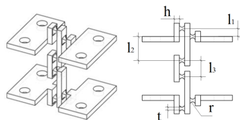
Fig. 7 Centring flexure hinge
