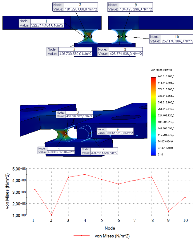
Fig. 11 Finite element analysis of the von Mises stress in the tilting flexure hinge
