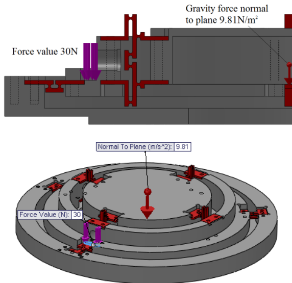
Fig. 8 Boundary conditions of tilting simulation study
