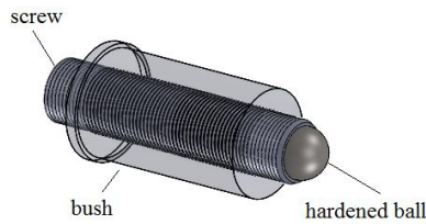
Fig. 4 Ultra fine adjustment screw
