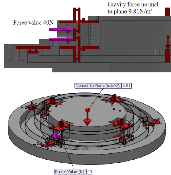
Fig. 9 Boundary conditions of centring simulation study
