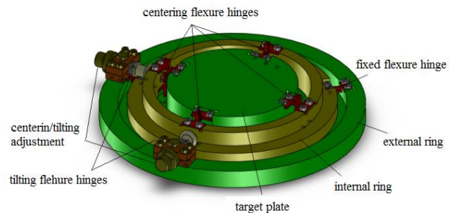
Fig. 1 4 DOF precise positioning stage
