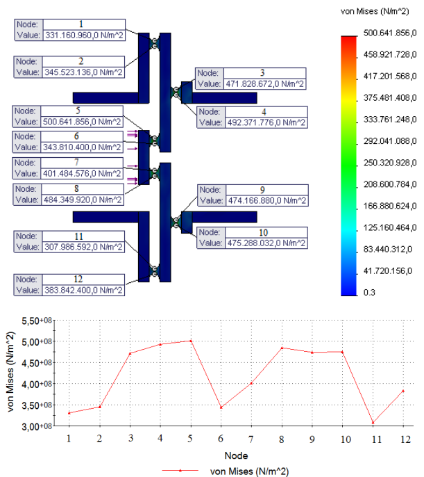
Fig. 13 Finite element analysis of the von Mises stress in the centring flexure hinge
