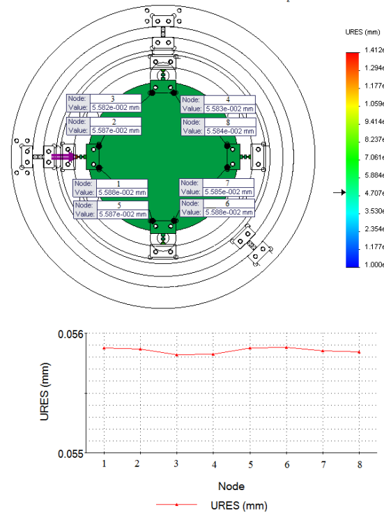
Fig. 12 Centring displacement simulation results when maximum input force was applied
