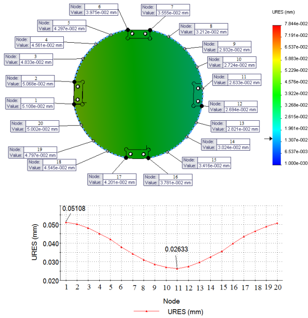
Fig. 10 Tilting displacement simulation results when maximum input displacement was applied
