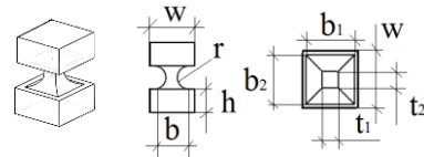
Fig. 5 Two-axis circular flexure hinge
