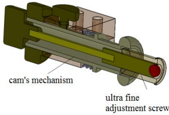
Fig. 3 Centring/tilting adjustment mechanism
