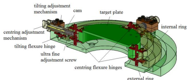
Fig. 2 Stage cross-section
