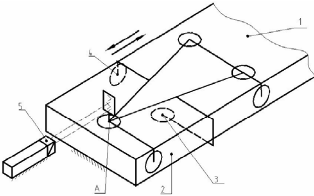
Fig. 1 Unit of linear movement with aerostatic bearings
