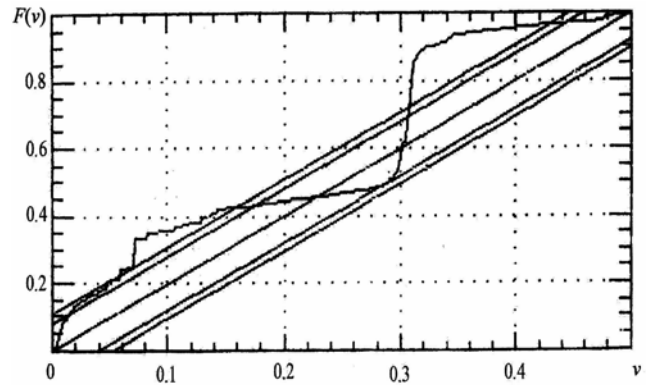
Fig. 4 Integrated period-diagram F(\nu) of motion errors for assembly with rolling bearings
