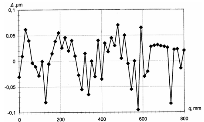
Fig. 8 Deviations of motion straightness errors from low frequency form errors of guideway on the displacement q for the assembly with aerostatic bearings
