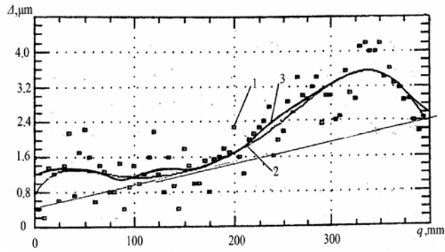
Fig. 5 Deviations of motion straightness (1), their approximation by the algebraic polynomial (2) and guideway form error (3) diagrams for the assembly with rolling bearings
