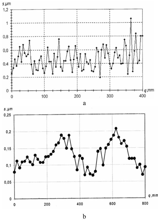
Fig. 2 Dependence of standard deviation in vertical plane on the displacement q for assemblies with rolling (a) and aerostatic (b) bearings
