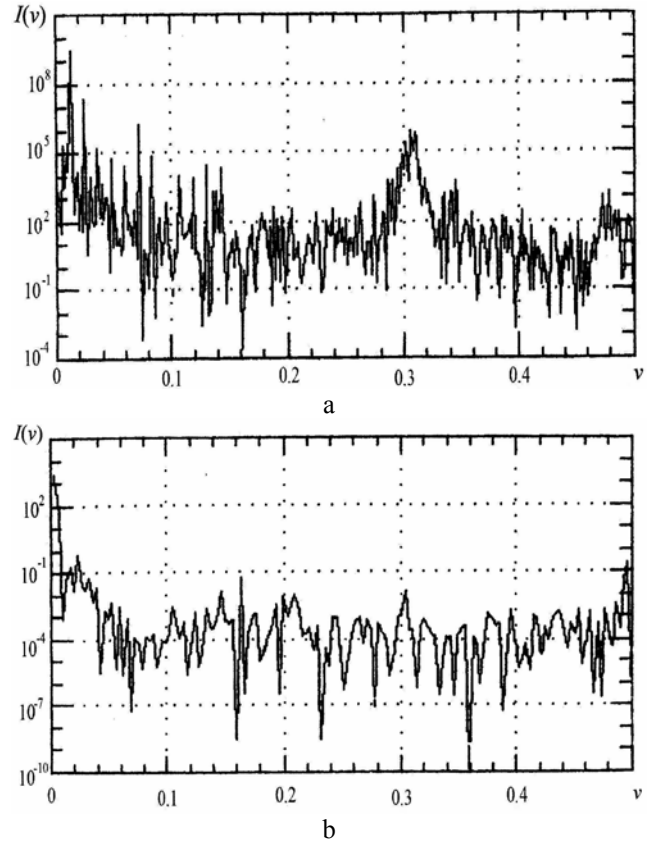
Fig. 3 Period-diagrams I(\nu) of motion errors for assemblies with rolling (a) and aerostatic (b) bearings
