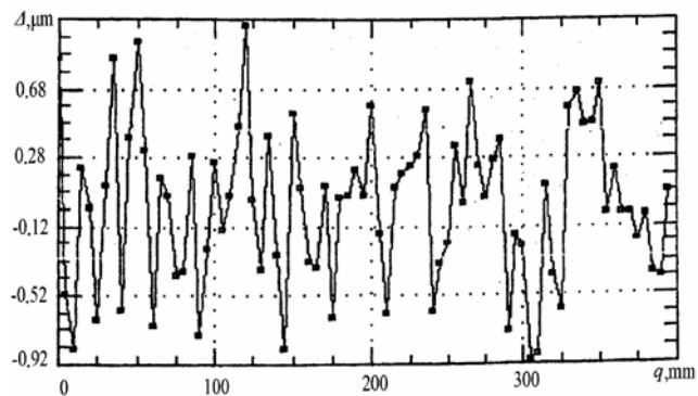
Fig. 6 Dependence of high frequency error of motion straightness on the displacement q
