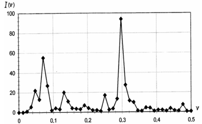
Fig. 7 Period-diagram I(\nu) of one realization of motion straightness errors for the assembly with rolling bearings
