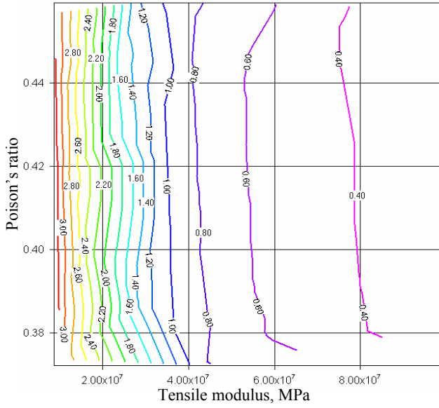
Fig. 7 Objective function landscape, where isolines show tube displacement values in mm
