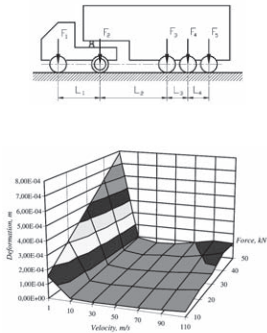
Fig 8. Interaction between a motor vehicle wheel and road surface (M. Bogdevičius) [4]
