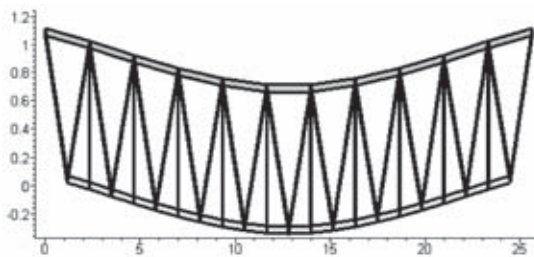
Fig 5. Research into the dynamics of overhead crane (M. Bogdevičius, A. Vika) [1]
