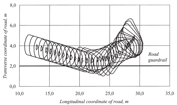
Fig 10. Interaction between a motor vehicle and road guardrails (O. Prentkovskis, M. Bogdevičius) [6]
