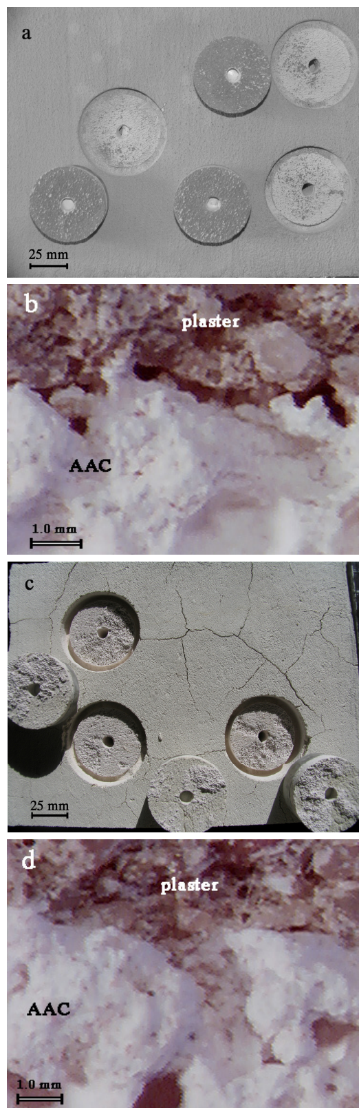
Fig. 6. Samples after measuring of force of adhesion to AAC base (a and c) and section of adhesion zone (b and d). a and b – reference samples, c and d – samples with 15 % zeolite additive
