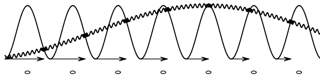
Fig. 1. Schematic picture of dislocation. Two layers of the crystal lattice. The position of the atoms of the bottom layer is marked by circles (o). The influence on the atoms of the upper layer (•) is reduced to the effect of potential energy (7). The interaction of atoms of the upper layer could be as usual described by spring interaction. Arrays show the corresponding displacements.
