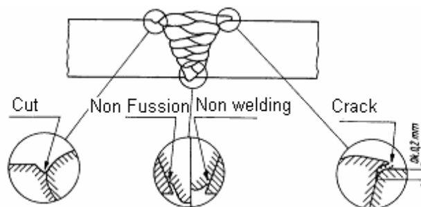
Fig. 1 The places for stress concentration in the welded joint, which can contribute to crack formation in the seam
