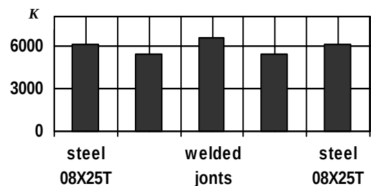
Fig. 7 Distribution of reliability in the welded joint welding grade 08X25T steels by austenitic-ferritic UTP-65D electrodes
