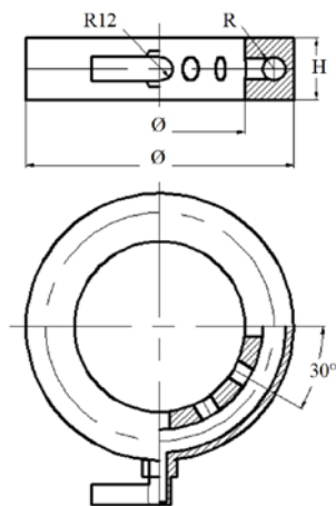
Fig.4. Universal plate
