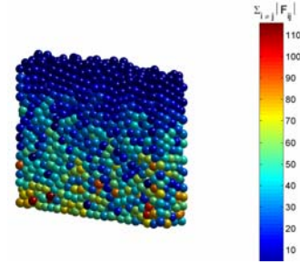
Fig. 6 Assembly of particles ( \mu=0.3 ) and the particle forces (measured in N )
