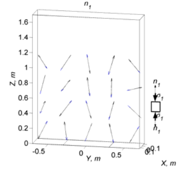
Fig. 10 Trajectories of the principal stress \sigma_1 ( \mu=0.3 )
