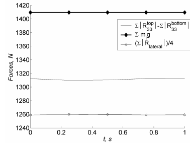
Fig. 7 Forces vs time ( \mu=0.3 )
