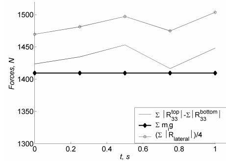
Fig. 4 Forces vs time ( \mu=0 )
