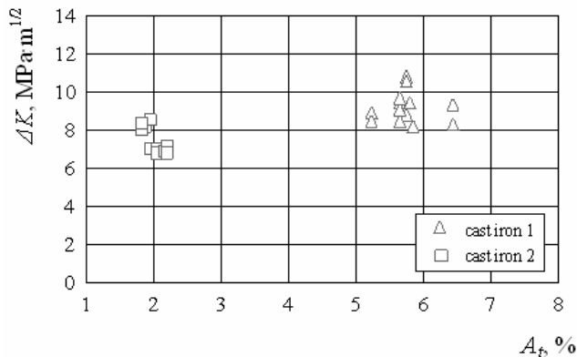
Fig. 6 Threshold stress intensity factor range \Delta K_{th} dependence on plasticity factor A_t
