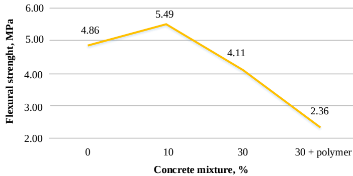
Fig. 4. Flexural strength of specimens.
