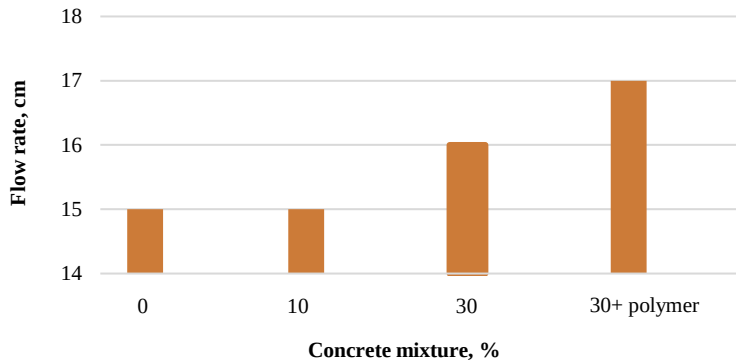
Fig. 3. Fresh concrete flow.
