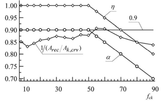
Fig. 4 Variation of 1/(A_{rec}/A_{crv}) ratio and coefficients \alpha and \eta with characteristic concrete strength
