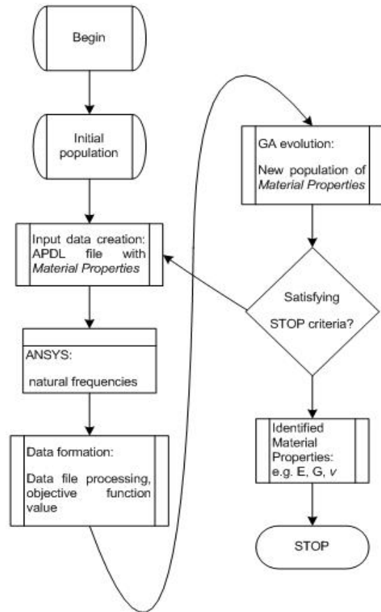
Fig. 4 Flow-chart for optimal design by GA
