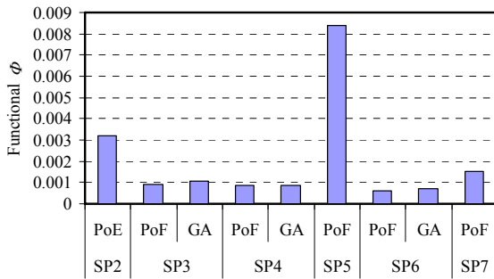
Fig. 7 Values of objective function using different identification techniques
