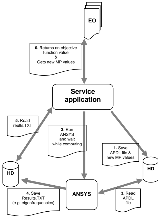
Fig. 3 Detailed optimization scheme
