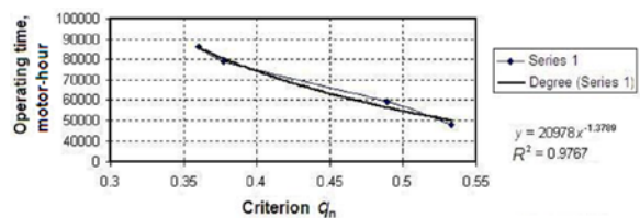
Fig. 3. Result of the adaptation of q_{II} criterion for diesel engines of Lithuanian Railways freight diesel locomotives
