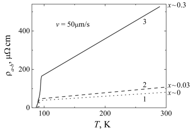
Fig. 4. Resistivity \rho_{a-b} vs. temperature dependences of YBCO devices containing an LW line produced using laser power of 0.22 W (curve #2) and 0.41 W (curve #3). Curve #1 is the reference, untreated device. Oxygen content x in the LW region (see the right y axis) has been extracted from [11], assuming a correlation between remnant oxygen content in defects/defect-free YBCO material and electric transport properties of oxygen-deficient YBCO films
