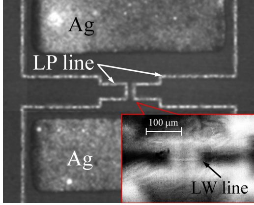
Fig. 2. A view of a YBCO thin film with LP (bright) insulating lines. Bright areas correspond to higher transparency of the light when a sample is illuminated from the bottom side. Inset: magneto-optical image of the penetration of the 280 G magnetic field into the superconducting device containing a single LW line. Bright areas in the inset correspond to higher intensity of a local magnetic field
