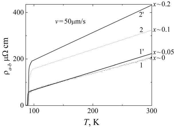
Fig. 5. The electric resistivity \rho_{a-b} vs. temperature dependences of two YBCO superconducting microbridges with the different initial content of oxygen: x \sim 0 (curve #1) and x \sim 0.1 (curve #2) and after the LW procedure with the laser power of 0.22 W: curves #1' and #2', respectively. The values of oxygen content x have been extracted from [11]
