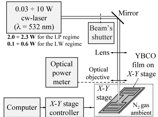
Fig. 1. The setup for LP and LW of the YBCO thin-film devices in a nitrogen gas ambient
