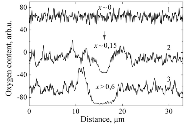
Fig. 3. The residual amount of oxygen vs. distance in three YBCO microbridges: without the LW region (curve #1), and the LW channel generated with the light power of 0.4 W and 0.6 W, (curve #2 and #3, respectively). For clarity, curves #1 and #3 are artificially shifted from zero position. A residual oxygen content x listed in the figure has been extracted from experimental results in [11]. The arrow in figure shows a approximate coordinate of the laser beam's center located on the bridges surface during the LW procedure
