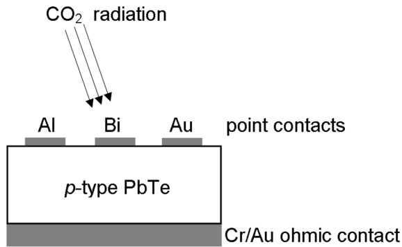
Fig. 1. Samples under investigation. CO 2 laser radiation is schematically shown falling separately on Bi-PbTe contact
