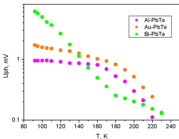
Fig. 3. Photoresponse signal across Al-, Au-, and Bi-PbTe Schottky contacts exposed to CO 2 laser radiation as a function of temperature
