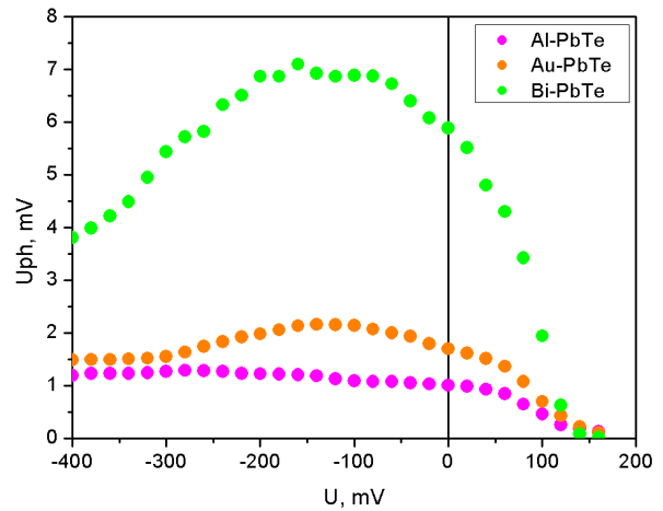
Fig. 2. Photoresponse signal across Al-, Au-, and Bi-PbTe Schottky contacts exposed to CO 2 laser radiation vs applied bias voltage at 92 K temperature
