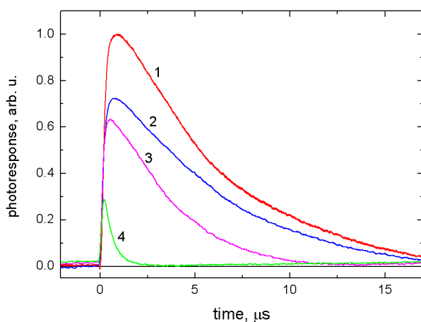
Fig. 4. Photoresponse signal pulses across Au-PbTe point contact exposed to CO 2 laser radiation at 92 K (1), 110 K (2), 140 K (3) and 200 K (4) temperature
