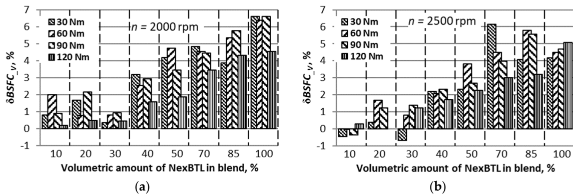
Figure 9. Relative deviation of BSFC according to volumetric fuel consumption [ml/kWh]: (a) n = 2000 rpm; (b) n = 2500 rpm.
