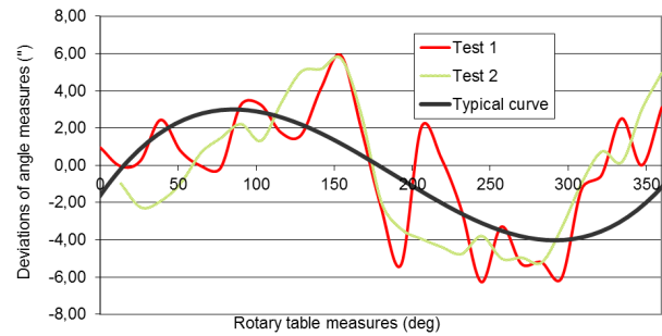
Fig. 3 Deviations of horizontal angle readings of Trimble 5503
