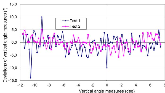
Fig. 5 Deviations of vertical angle readings of Nikon DTM352
