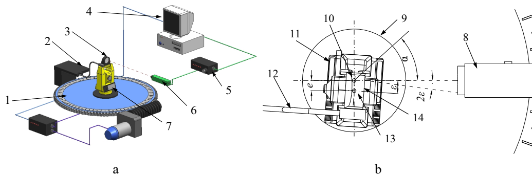
Fig. 1 Determination of angular position of calibrated device: a) general arrangement; b) principal diagram, 1, 9 – rotary table, 2, 12 – holder of calibrated device, 3, 14 – position determination mirror, 4 – PC, 5 – autocollimator control unit (optional), 6, 8 – position determination autocollimator, 7, 11 – calibrated geodetic device, 10 – centre of rotation of the rotary table, 13 – centre of rotation of calibrated device
