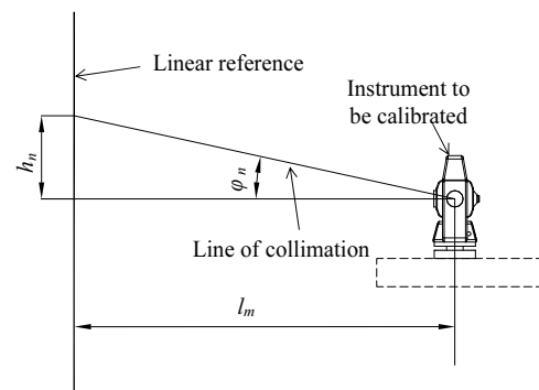
Fig. 2 Principle of trigonometric vertical angle measurement
