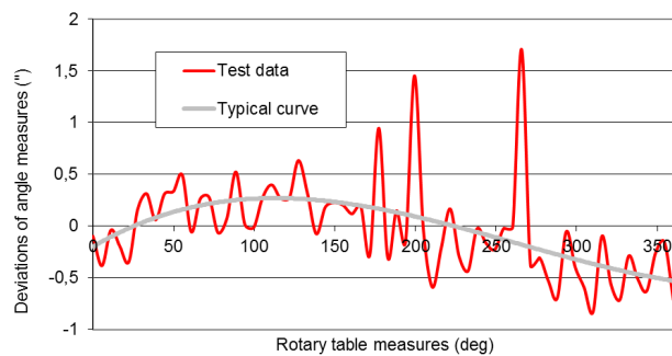
Fig. 4 Deviations of horizontal angle readings of Nikon DTM352
