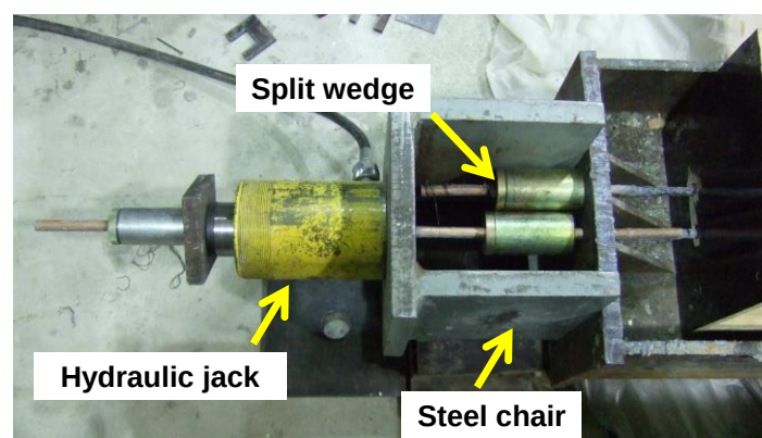
Figure 3. Jacking setup.
