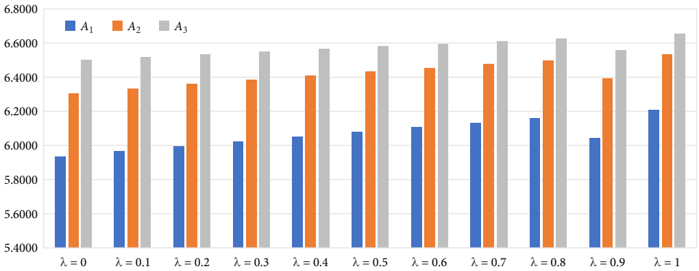
Figure 1. Sensitivity analysis results for different values of \lambda
