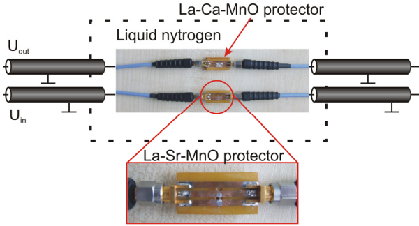
Fig. 3. Outside view of two-stage protector
