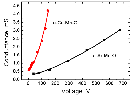
Fig. 4. Conductance vs. voltage across the samples of La-Ca(Sr)-Mn-O films
