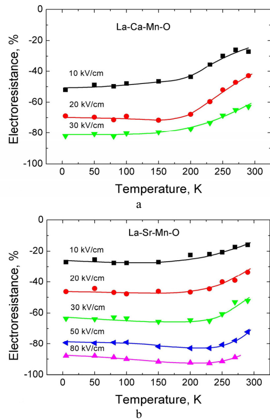
Fig. 5. Electroresistance vs. temperature dependences at different electrical field strengths for La-Ca-Mn-O (a) and La-Sr-Mn-O (b) films
