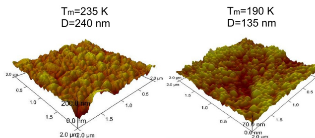
Fig. 1. Atomic Force Microscopy images of La-Sr-Mn-O (left) and La-Ca-Mn-O (right) films
