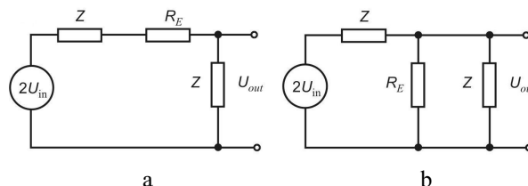
Fig. 2. Equivalent circuit for investigation of the ER of polycrystalline films (a) and transient characteristics of the protector (b). R_E is resistance of the sample, 2U_{in} is voltage from the generator, U_{out} is voltage measured across input impedance of oscilloscope Z = 50 \Omega
