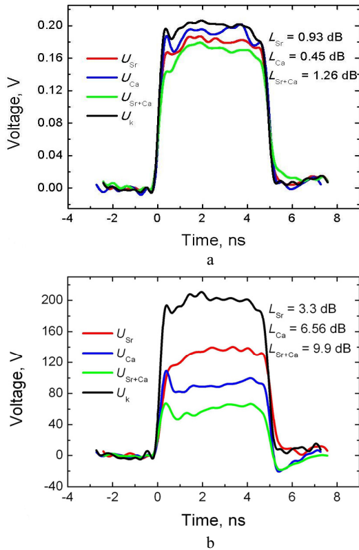
Fig. 6. Transient waveforms of La-Ca-Mn-O protector, La-Sr-Mn-O protector and two-stage protector operating at T = 80 K in non-limiting (a) and limiting (b) regimes
