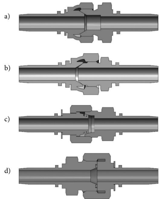
Figure 3. Cross-section standards of 3D model fitting connections: a – BSP; b – JIS; c – DKOL; d – ORFS
