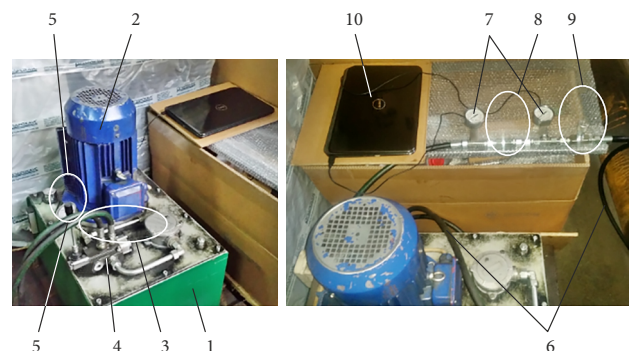
Figure 5. The experimental bench for investigating pressure losses at fitting connections
