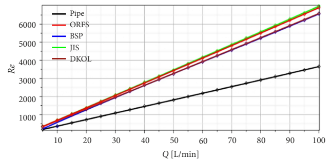
Figure 9. The chart of in depending Re number from flow rate for different fitting connections
