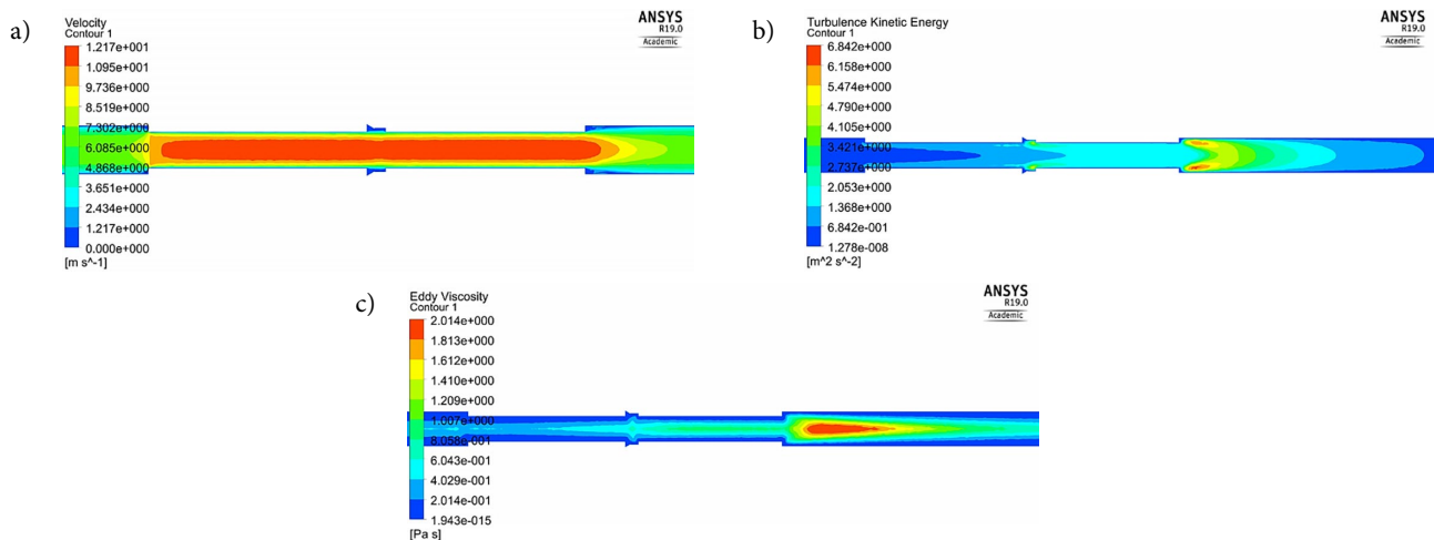
Figure 11. Additional results from the fluent simulation of the DKOL fitting connection: a – velocity; b – turbulence kinetic energy; c – eddy viscosity
