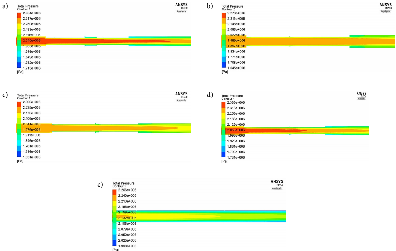
Figure 10. Total fluid pressure across fitting connections (by fluent simulation): a – BSP fitting connection; b – JIS fitting connection; c – DKOL fitting connection; d – ORFS fitting connection; e – straight pipeline of the equivalent length
