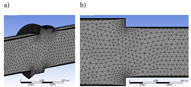
Figure 7. The mesh of the model: a – mesh generation; b – inflating layers with the expansion factor of 1.2...1.6
