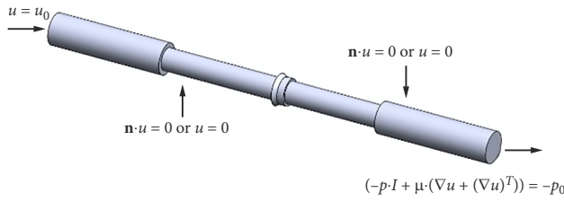
Figure 6. Boundary conditions of the pipeline-fittings system for Ansys® Fluent® simulation
