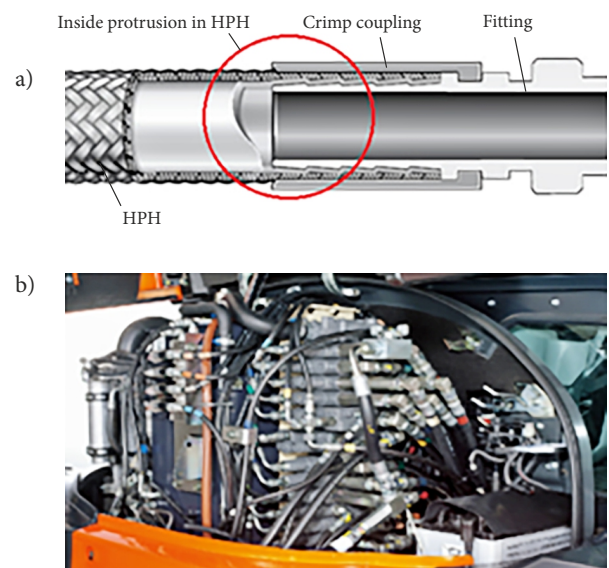
Figure 1. The typical hydraulic composition of a system (Karpenko, Bogdevičius 2018):
