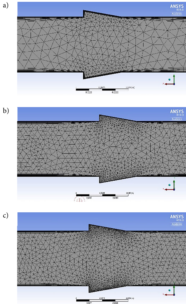
Figure 8. Mesh resolution of the mesh independence study: a – M1; b – M3; c – M5
