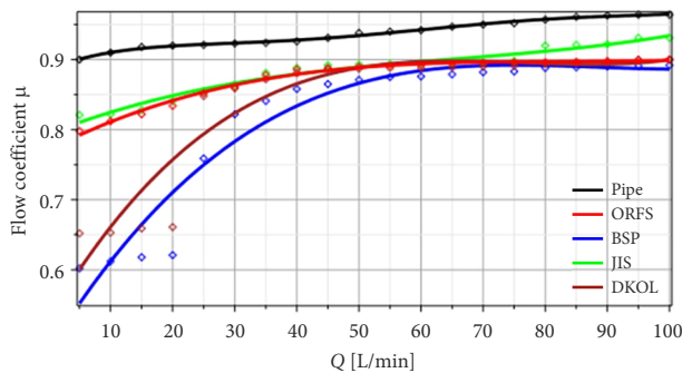
Figure 12. A chart of the flow coefficient at a different flow rate of fitting connections
