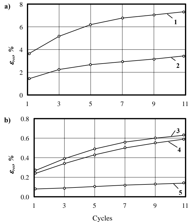
Fig. 2. The development of residual deformations in expanded polystyrene with the density of 14 \text{ kg/m}^3 : a – under cycling compressive stress equal to: 1 – \sigma_{10} ; 2 – \sigma_5 , b – the same for: 3 – 1.2\sigma_{cr} ; 4 – \sigma_{cr} ; 5 – 0.8\sigma_{cr}
