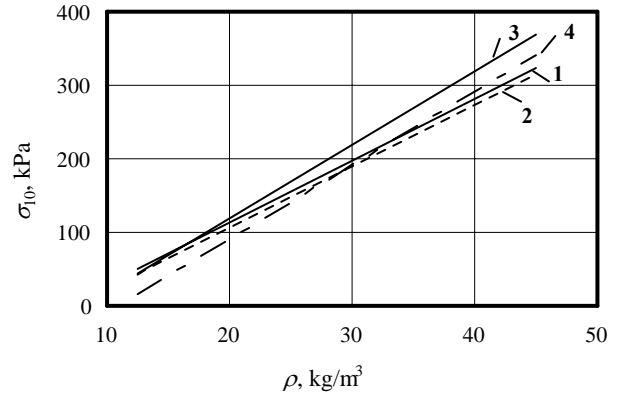
Fig. 4. The empirical lines of the values of stress corresponding to 10 % deformation of expanded polystyrene slabs under compression, depending on their density. Lines 1, 2 – mean and predicted stress values for slabs manufactured by Lithuanian enterprises; 3, 4 – the same according to the data provided in [7]
