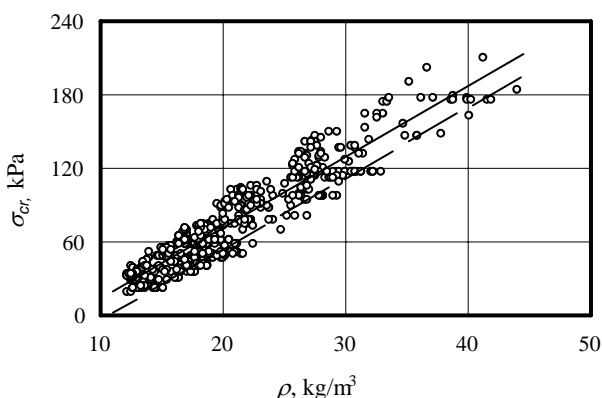
Fig. 5. The dependence of the critical stress developed in expanded polystyrene slabs under compression on their density. o – experimental values; the continuous line – the empirical regression line of the critical stress value according to slab density; the dotted line – the same for the predicted stress value according to slab density
