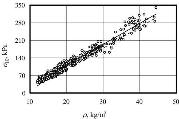
Fig. 3. The stress corresponding to 10 % deformation of expanded polystyrene slabs under compression, depending on their density. \circ – experimental values; the continuous line – the empirical regression line of the mean stress value according to slab density; the dotted line – the same for the predicted stress value according to the slab density
