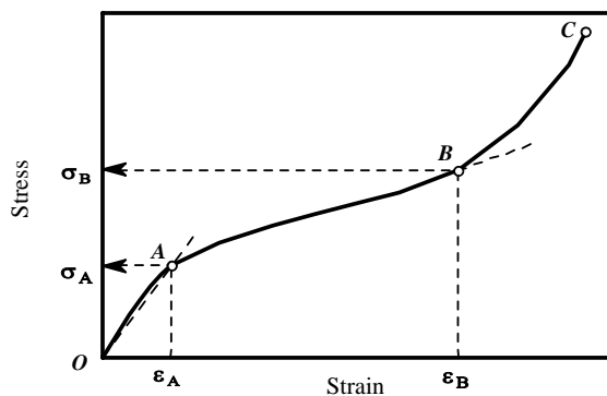
Fig. 1. A scheme of expanded polystyrene under short-term compression [3–5]
