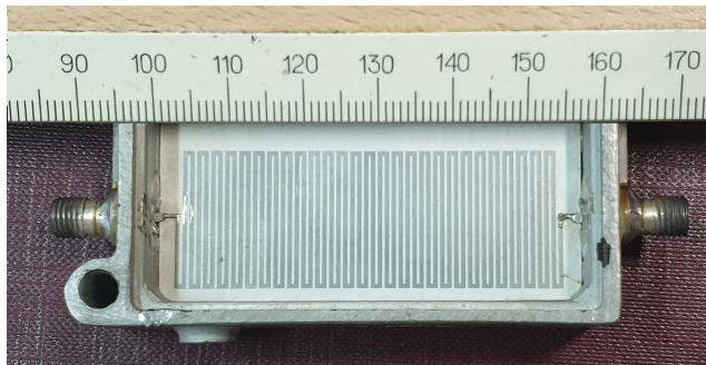
FIGURE 2. Experimental layout meander microstrip delay line.
