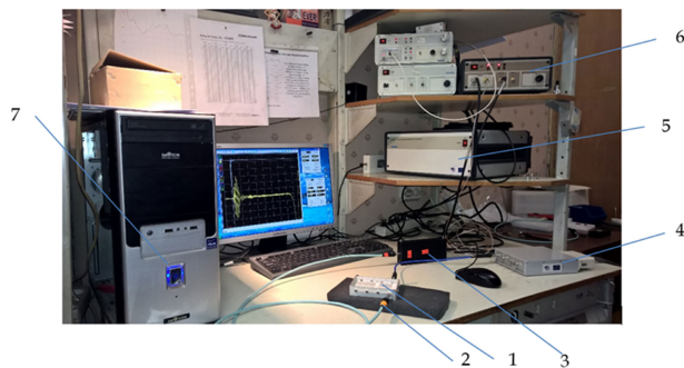
FIGURE 3. A block diagram of an experimental measurement of the delay time of a prototype of the meander microstrip line (a), and a general photograph of the experiment (b); where 1 is the meander delay line-under-test, 2 is the attenuator, 3 is the pulse shaper GZ117GN-03, 4 is the sampling unit SU-3130, 5 is the digital sampling precision converter SD20037, 6 is the pulse generator mainframe GZ-1106DL2, 7 is the computer with the control software.
