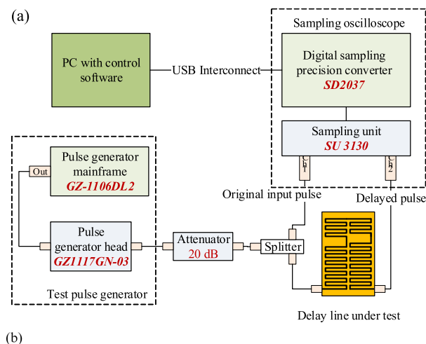
FIGURE 2. Experimental layout meander microstrip delay line.
