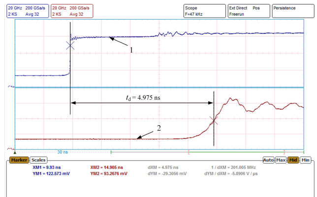
FIGURE 6. An example of signals of input and output pulses of the meander microstrip line, here 1 – pulse at the input of the delay line; 2 – pulse at the output of the delay line, delay time 4.975 ns.
