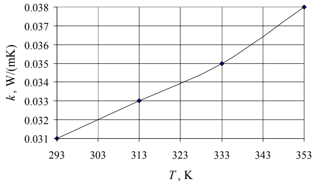
Fig. 2 Temperature dependent conductivity of polyurethane insulation
