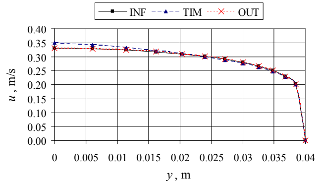
Fig. 3 Distribution of the velocity: boundary conditions at the inflow (INF); computed velocity profile at the outflow, when t=300 s (OUT); computed velocity profile at the outflow, when t=9 s (TIM)
