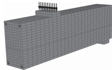
Fig 8. The finite element model used in numerical analysis by software MSC.Marc
