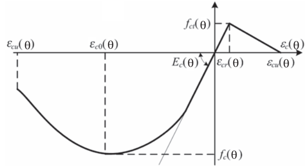
Fig 4. Model of stress-strain relationship of concrete
