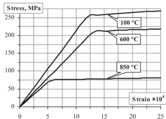
Fig 6. Idealization of stress-strain behaviour for steel at elevated temperatures
