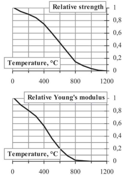
Fig 5. Reduction coefficients allowing for decrease of concrete compressive strength and Young's modulus at elevated temperatures
