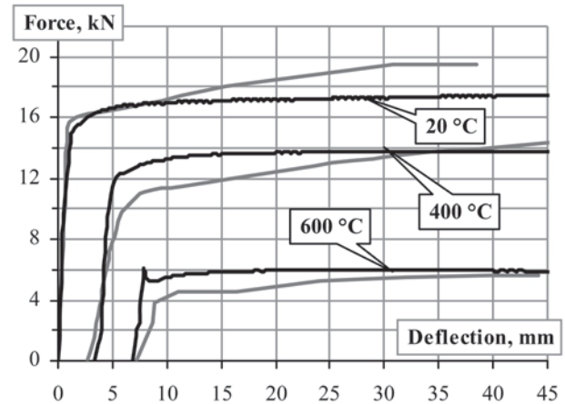
Fig 11. Experimental (grey curve) and calculated (black curve) load-deflection diagrams
