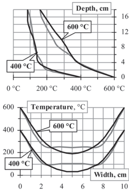
Fig 10. Experimental (grey curve) and calculated (black curve) temperature distribution along (above) and across section (below) of the beams exposed to 400 °C and 600 °C
