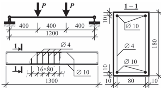
Fig 2. The loading configurations and specimen dimensions
