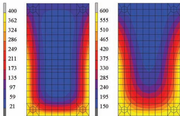
Fig 9. Calculated temperature distribution in a cross-section of the beams exposed to temperatures 400 °C (left) and 600 °C (right) achieved after 4,5 and 20 min heating, respectively
