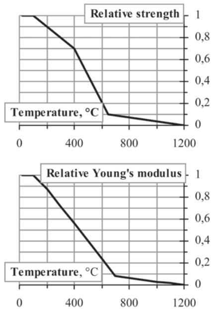
Fig 7. Reduction of strength and Young's modulus of steel at elevated temperatures
