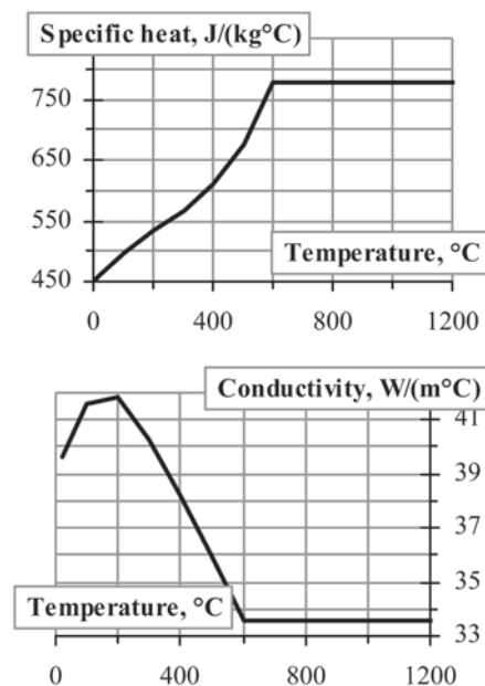
Fig 3. The specific heat and the thermal conductivity of reinforcement steel
