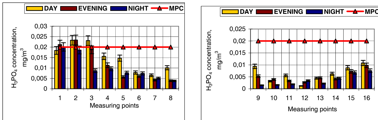
Fig 9. Phosphorus acid concentration 10–50 m and 200–300 m from AB KLASCO territory in July
