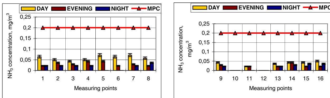
Fig 7. Ammonia concentration 10–50 m and 200–300 m from AB KLASCO territory in November
