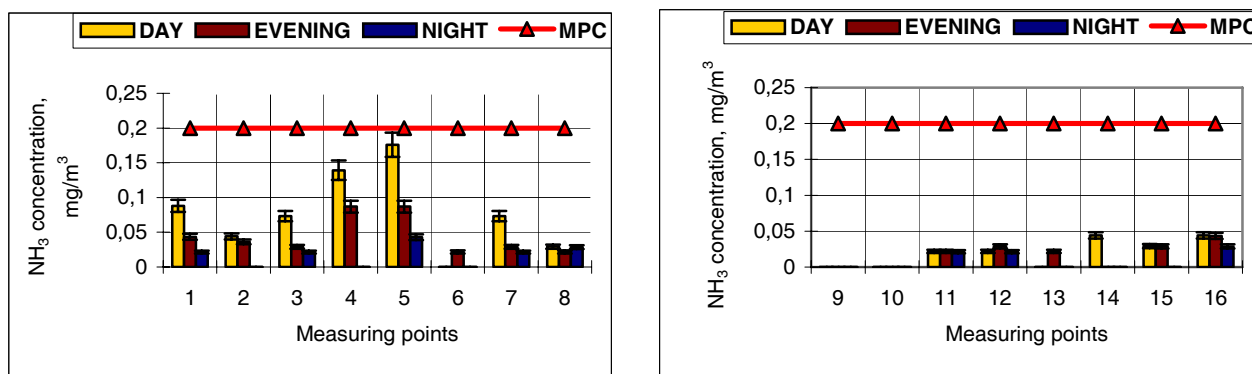
Fig 6. Ammonia concentration 10–50 m and 200–300 m from AB KLASCO territory in October
