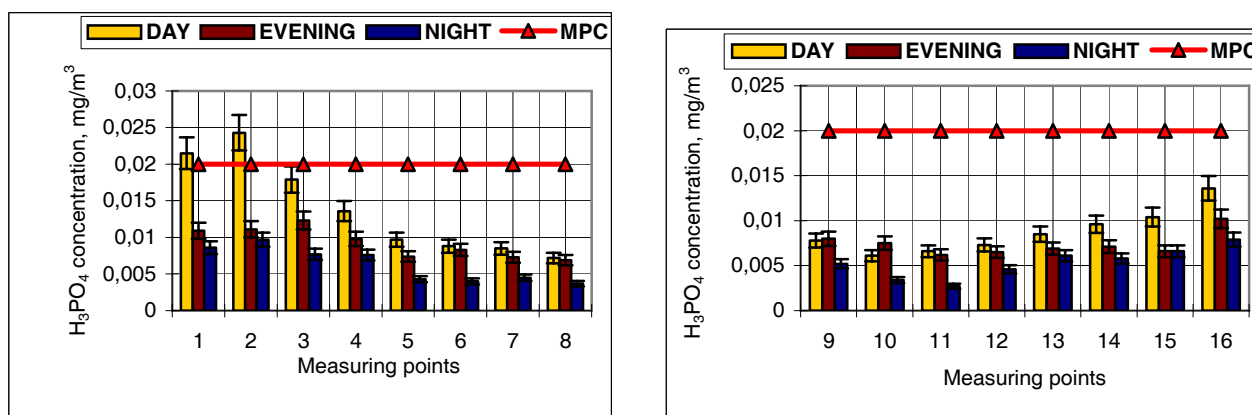
Fig 8. Phosphorus acid concentration 10–50 m and 200–300 m from AB KLASCO territory in June
