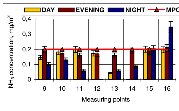
Fig 2. Ammonia concentration 10–50 m and 200–300 m from AB KLASCO territory in June
