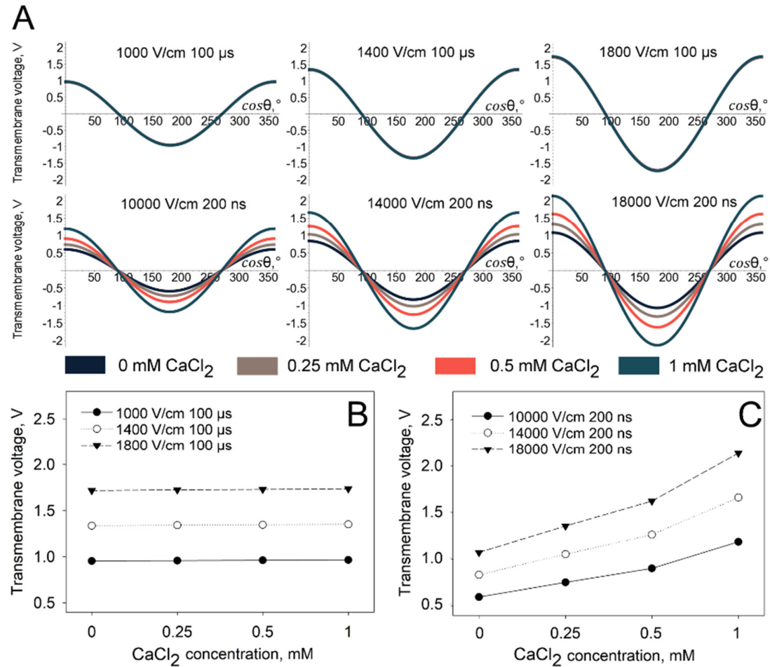
Figure 8. Modelling of transmembrane potential distribution on cell surface (A) and the peak transmembrane potential at the electrode-facing poles after microsecond (B) and nanosecond (C) electric pulse treatment.
