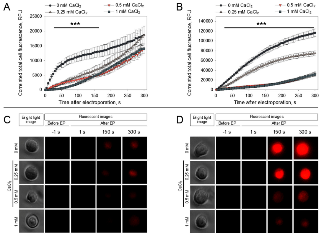
Figure 6. Visualization of PI electrotransfer into cells in media with different CaCl 2 concentrations. The cells were electroporated with single 1400 V/cm (A) or 1800 V/cm (B) strength, 100 \mu s duration electric pulses. Electroporation was performed at time '0 s'. The fluorescent images in panels (C) and (D) represent key points images from the (A) and (B) panels, respectively. Statistical differences (A and B) of PI uptake between control (0 mM CaCl 2 ) and 0.25; 0.5; 1 mM CaCl 2 are denoted by ***— p < 0.001 . The error represents the mean \pm standard error of mean of n = 20 experimental replicates.
