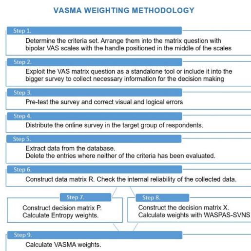
Figure 2. VASMA weighting methodology.
