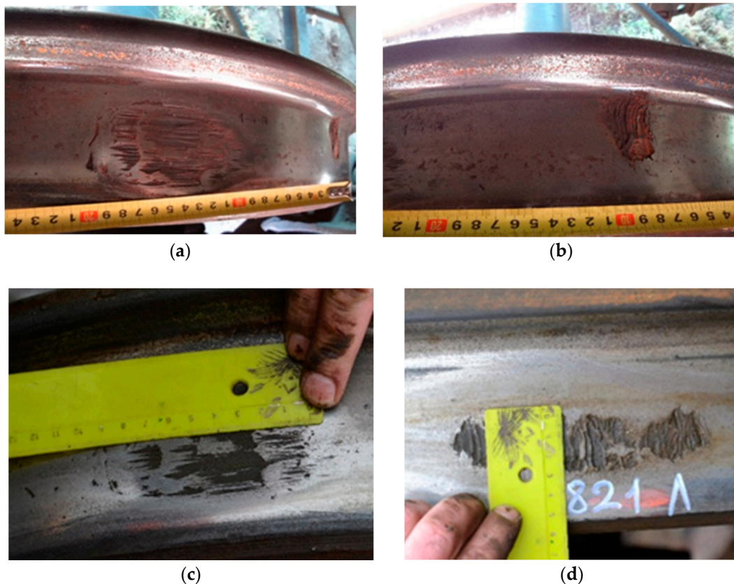
Figure 8. Wheel with surface unevenness ((a–d)—flat spot)—unevenness 4.
