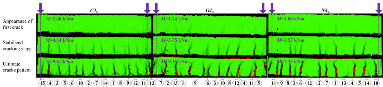
Figure 2. Cracking schemes identified by the DIC system
