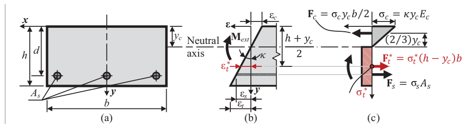
Figure 4. Analytical model of the element subjected to external bending moment M_{ext} : a) RC section; b) strain profile; c) stresses and internal forces acting in section
