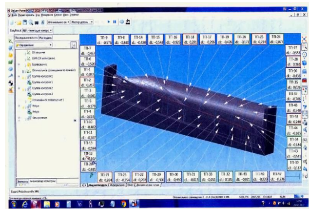
Fig. 1. Results of the measurement of the surface of the aircraft component with the determination of the error and deviation of the form
