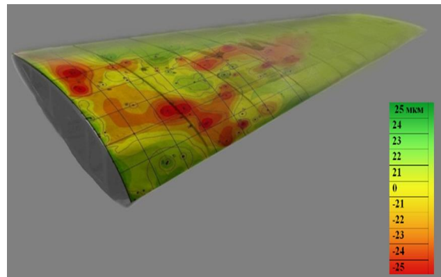
Fig. 2. Color map of geometric parameters of deviation from the shape and location of the surface
