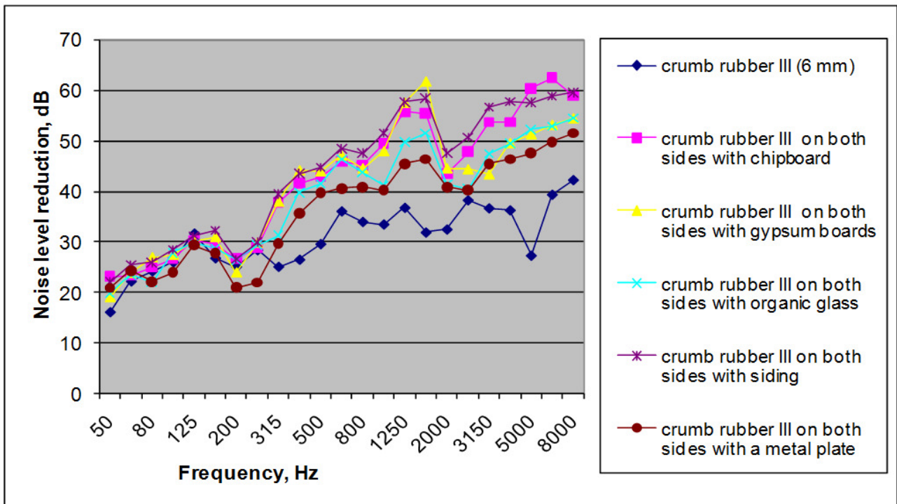
Fig 4. Results of noise level reduction in the samples of experimental structures
