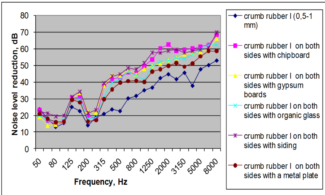
Fig 2. Results of noise level reduction in the samples of experimental structures
