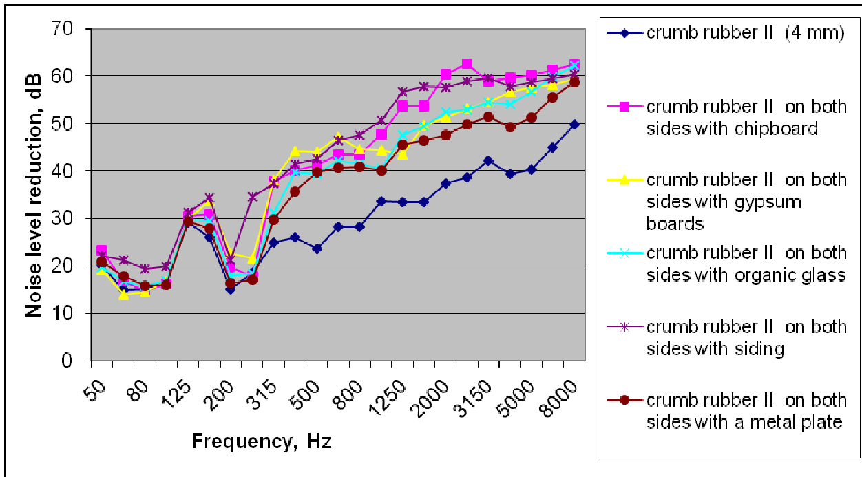
Fig 3. Results of noise level reduction in the samples of experimental structures
