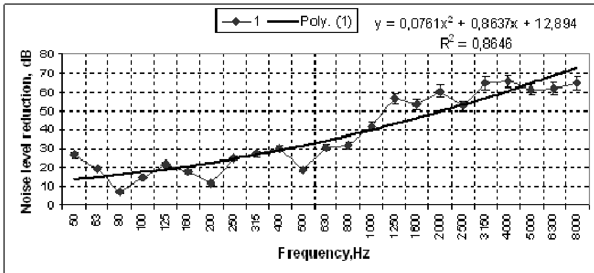
Fig 5. Noise level reduction in the sample of experimental structure 1
